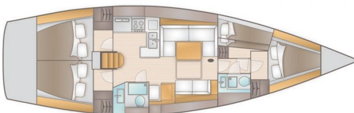
- Salona 44 layout
