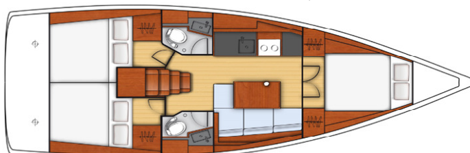
- Oceanis 38.1 layout
