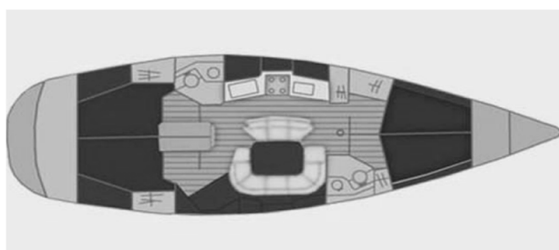
- Sun Odyssey 45.2(Topless express) Layout
